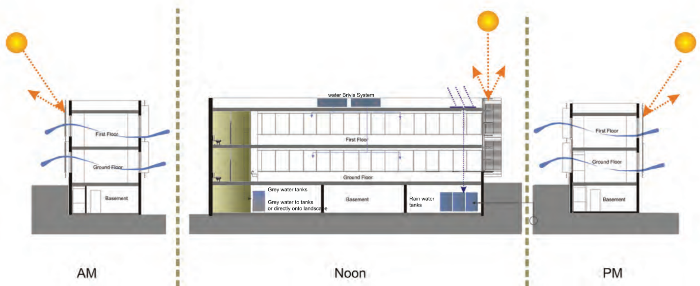
passive summer cooling water systems
